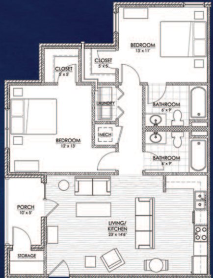
2 BR, 2 BATH FLOOR PLAN
